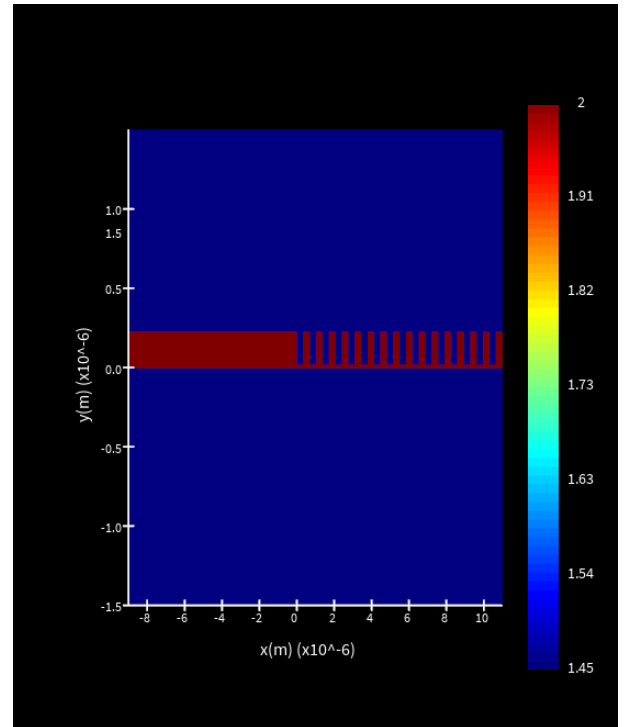
Fig. 5.3. Index-Monitor 1
