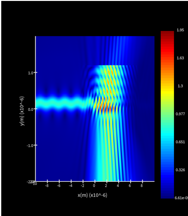
Fig. 5.2. Field-Monitor
