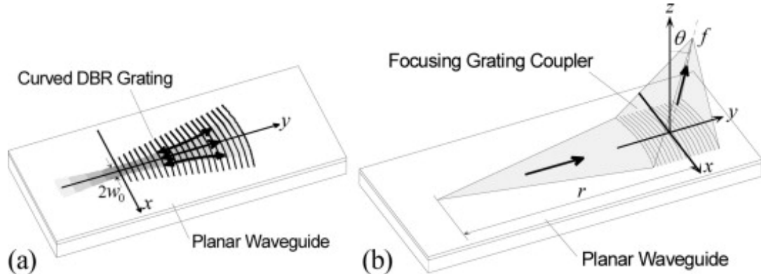
Fig. 6.1. Coned-GC [18]
