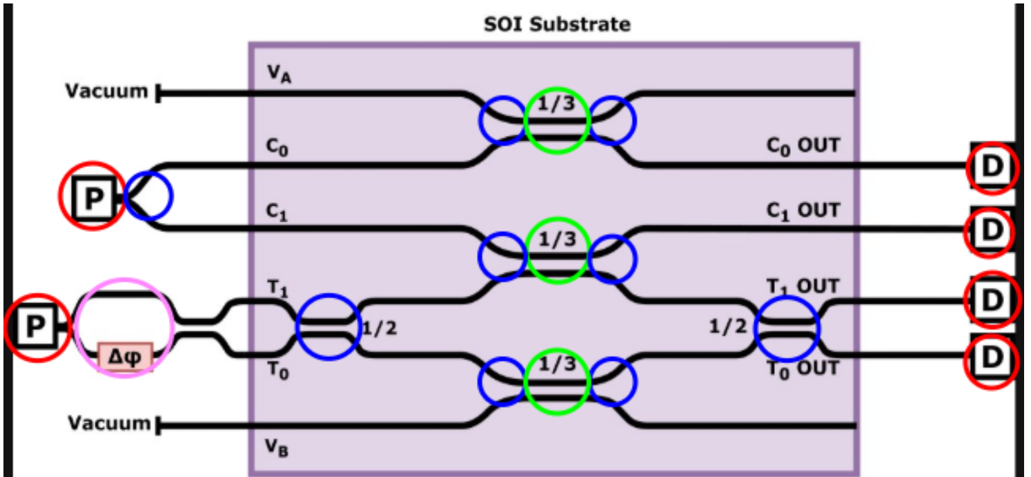
Fig. 4.1. 4x4 Unitary
