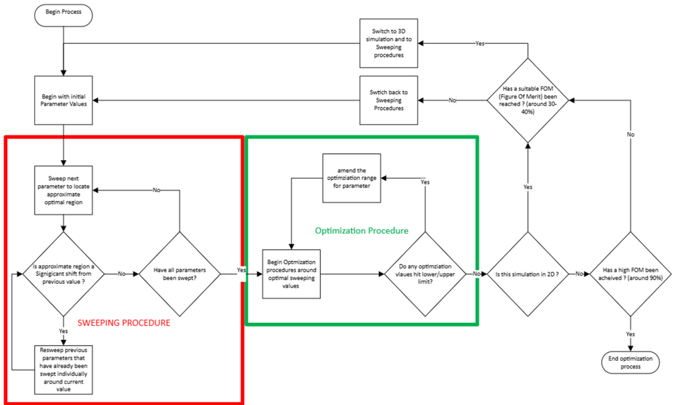
Fig. 5.9. Design-Flow
